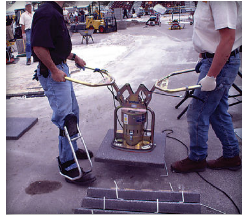
Figure 21. Vacuum assisted mechanical equipment for installing paving slabs.
