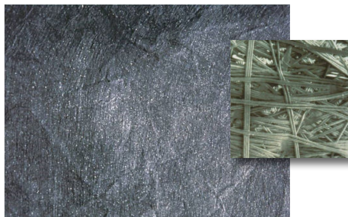
Figure 15. Non-woven heat bonded geotextile with close-up
