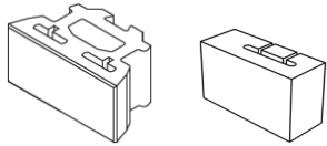
Standard Unit 8" x 18" x 10.125"
