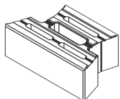
Stretcher Unit Face 1: 6" x 18" x 11" Face 2: 6" x 12" x 11"
